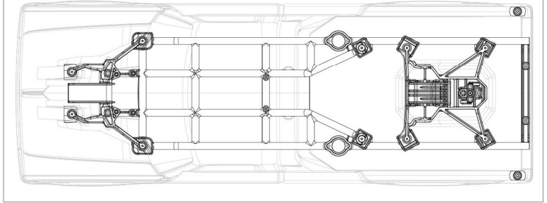
Completed Assembly (view from bottom)
