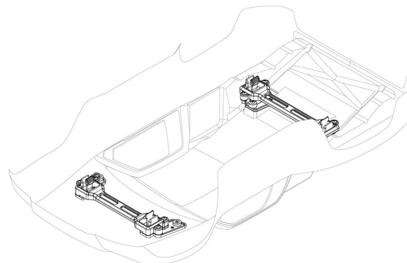
Completed Assembly (view from bottom)
