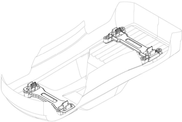
Completed Assembly (view from bottom)
