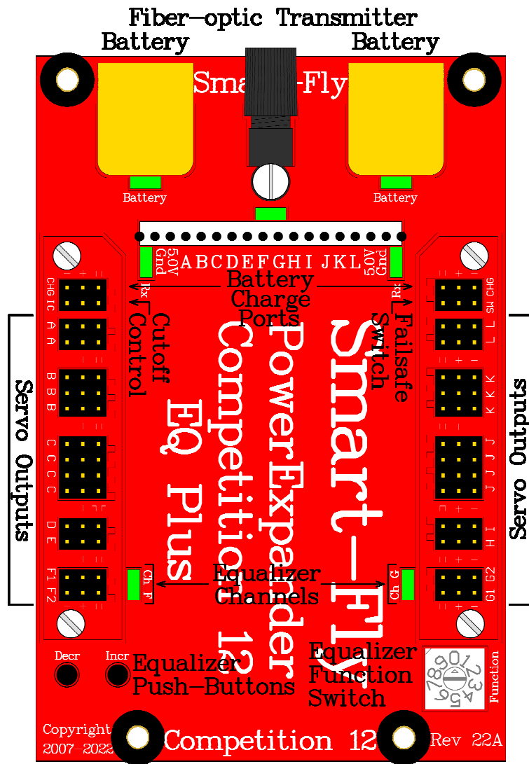
Reference Drawing
