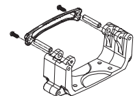
RER13447 - Front Suspension Mount & Pin Holder
