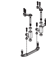
RER13435 - Steering Rack Assembly
