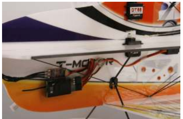
36. Connect servo and ESC to receiver, then power on and do equipment test.
